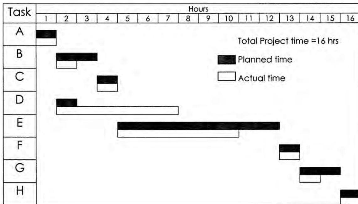
Figure 2.7.10 Bar chart indicating the planned as well as actual time taken in each repair activity of the electric motor
