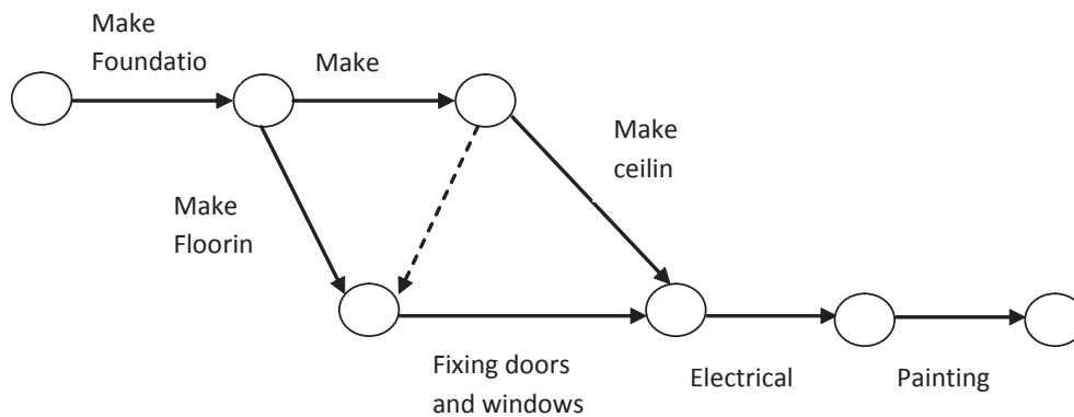
Fig. 2.7.18 Sequencing of activities in construction of building
