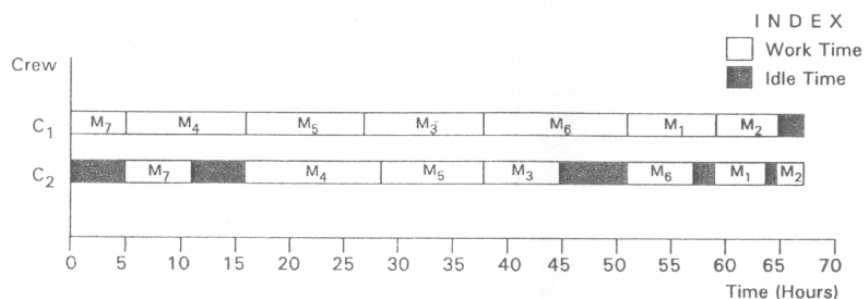
Fig. 2.8.10: Gantt Chart Showing Working of Crew
