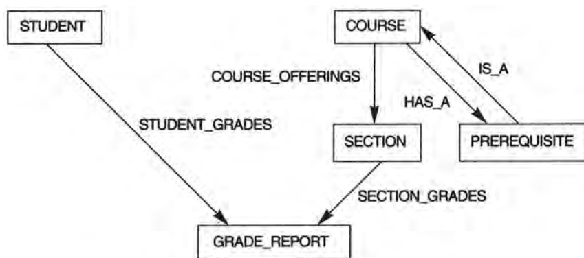
Fig. 9: The schema in the notation of the network data model
