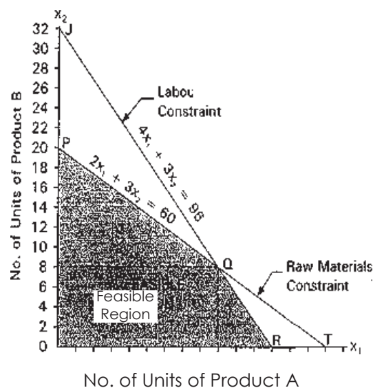
Fig. 2.10.16 Graphic Presentation of Constraints
