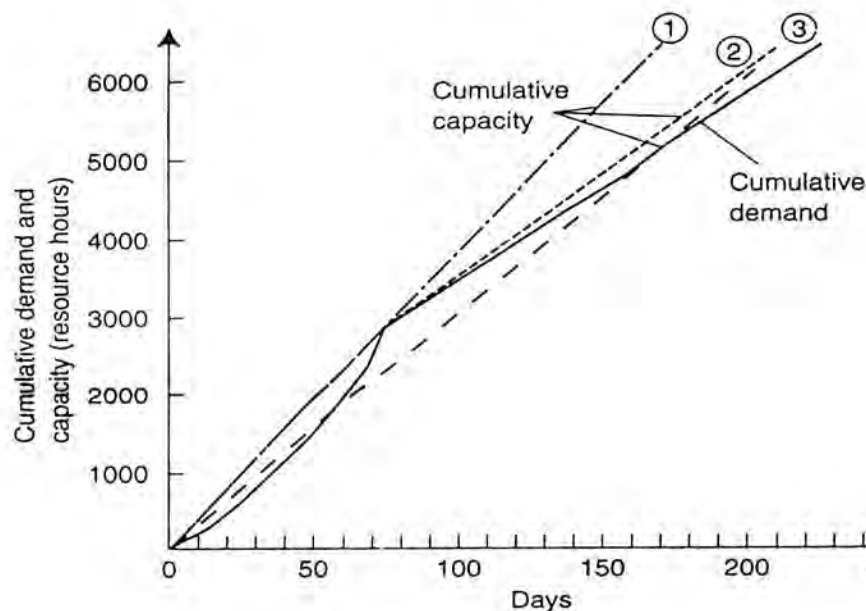
Fig. 2.5.14 Cumulative demand and capacity curves
