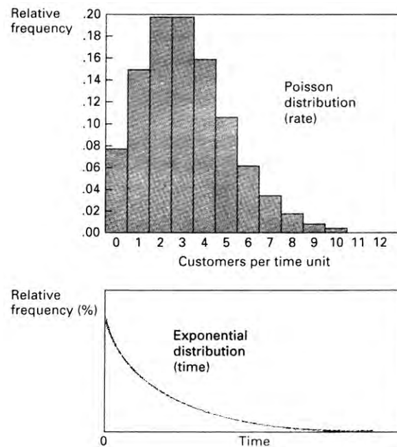
Fig. 2.8.5 Poisson and negative exponential distributions
