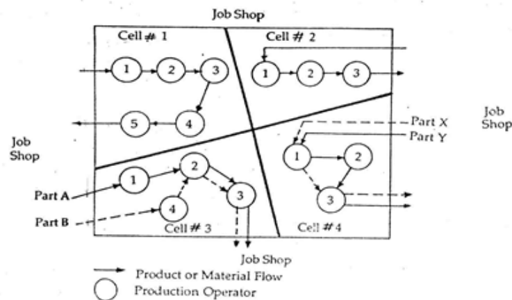
Fig. 2.6.4 Cellular Manufacturing
