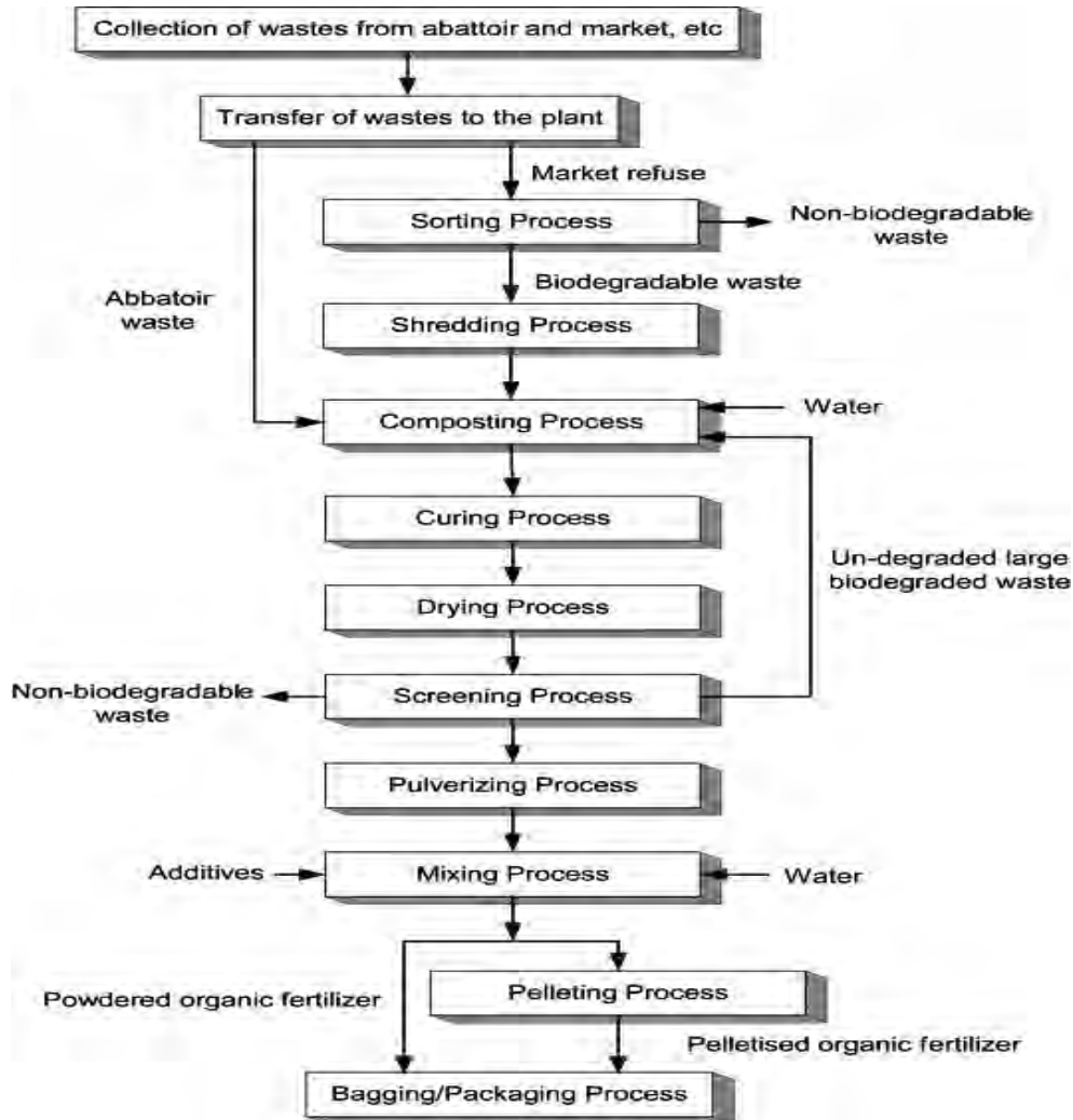
Fig. 32: Flowchart for Fertilizer
