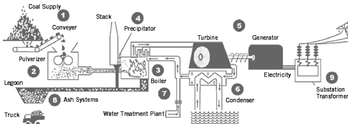
Fig. 39: Components of a thermal power plant
