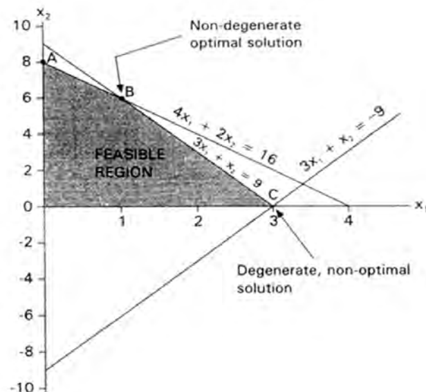
Fig. Graphic Solution: Non-degenerate, Optimal
