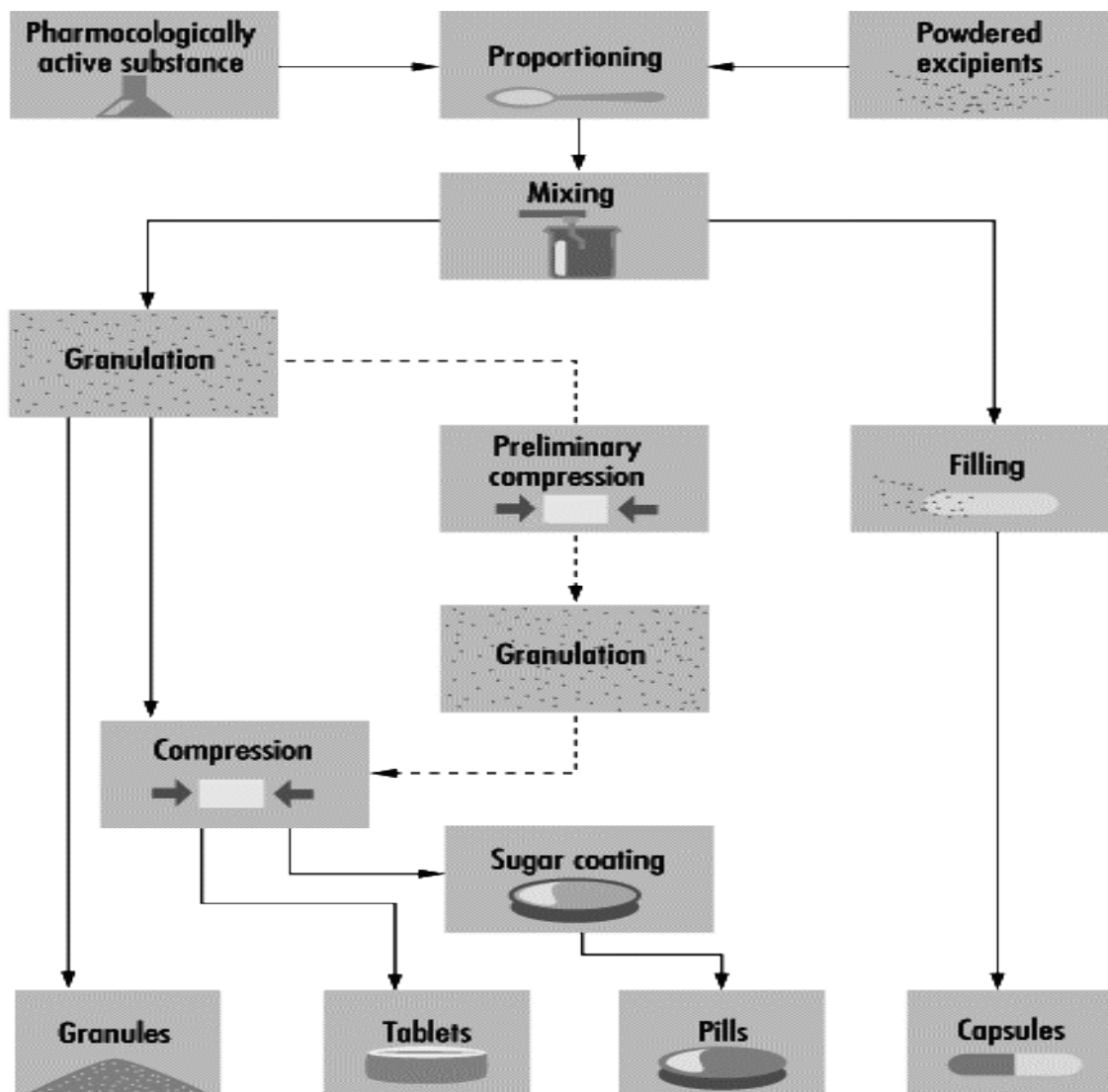
Fig. 36: Operations for Manufacturing of Pharmaceutical dosage form Products
