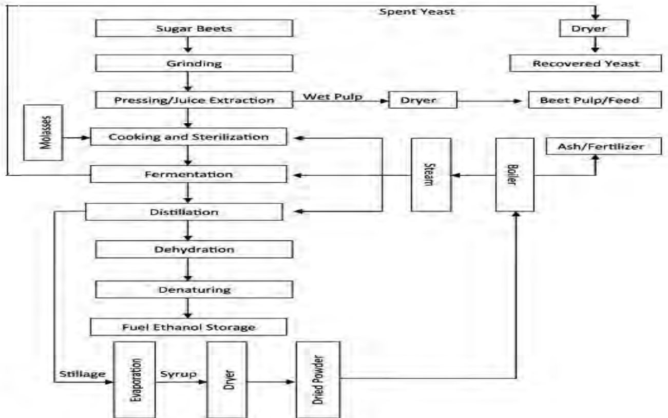
Fig. 31: Flowchart of Production Process for Industrial Alcohol
