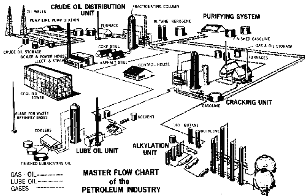
Fig. 37: Flowchart of Petroleum Industry
