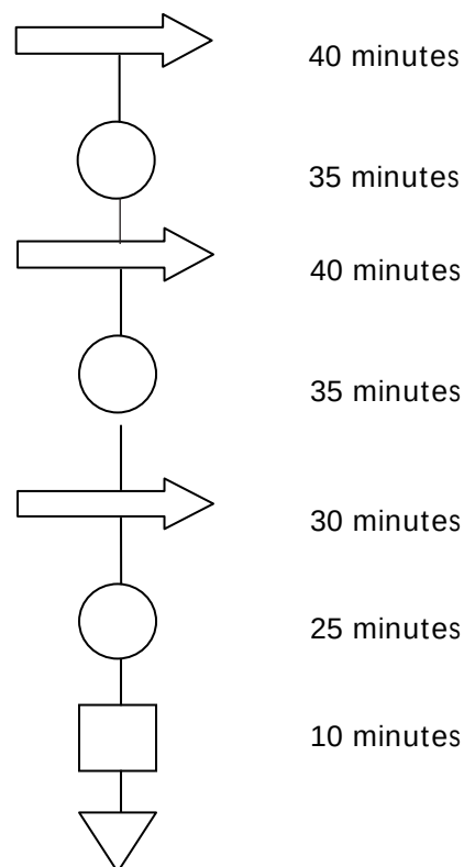
Fig. 23.3 Process Flow Chart
