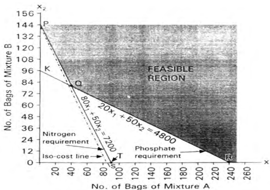
Fig. 2.10.4 Graphic Solution to the LLP
