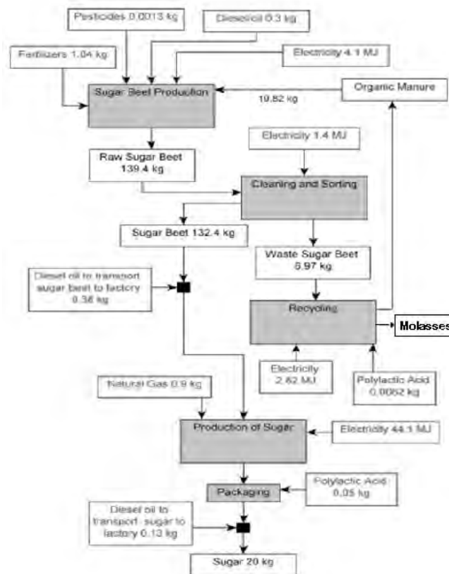
Fig. 30: Production Process of Sugar and Industrial Alcohol
