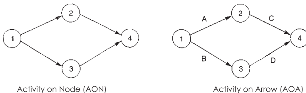
Fig. 2.7.14 Comparison of AON and AOA
