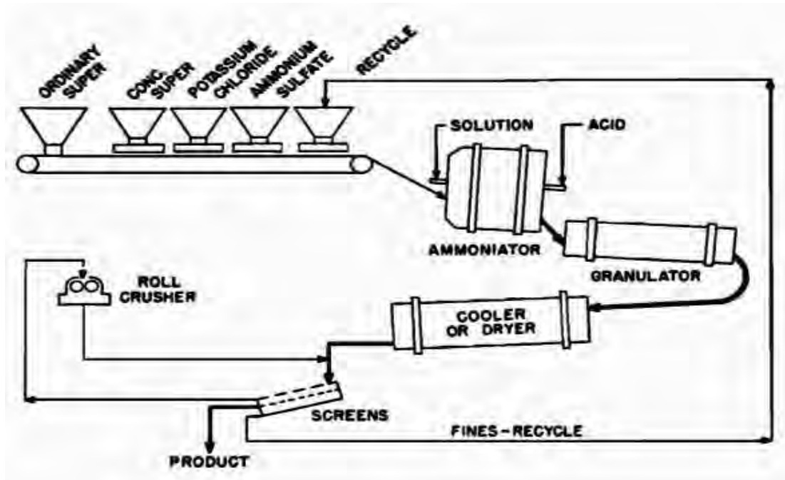
Fig. 34: Processing of General Fertilizer
