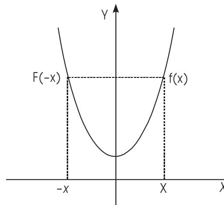
This graph is of the equation f(x)=x^2
