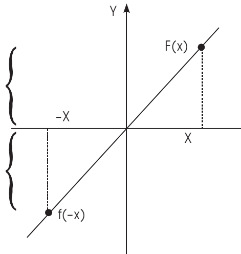
This graph is the equation of f(x)=x
