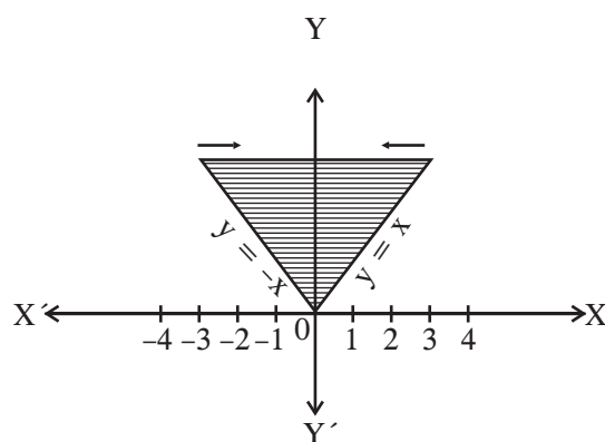
Graph of y \geq |x|
