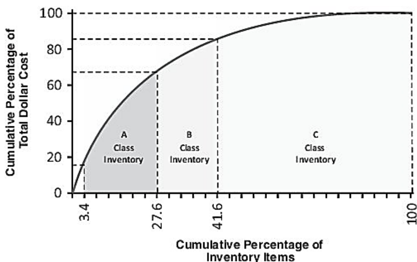
ABC ANALYSIS 21
