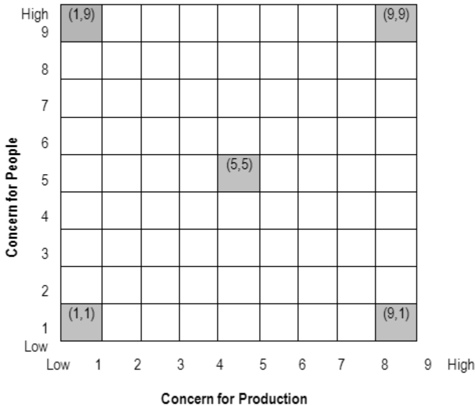
Figure 1: Managerial Grid
